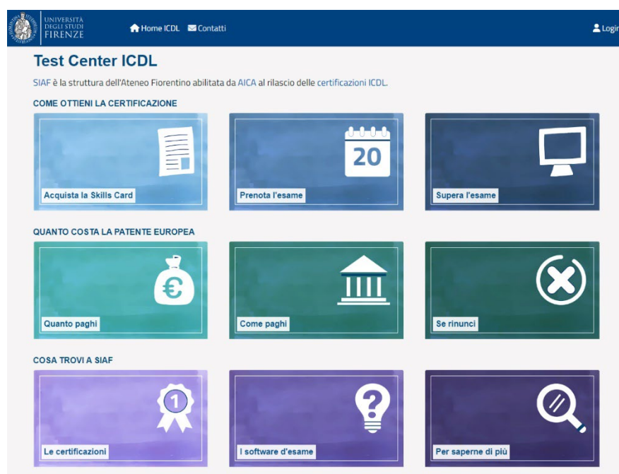
Figura 1 - ICDL Homepage
